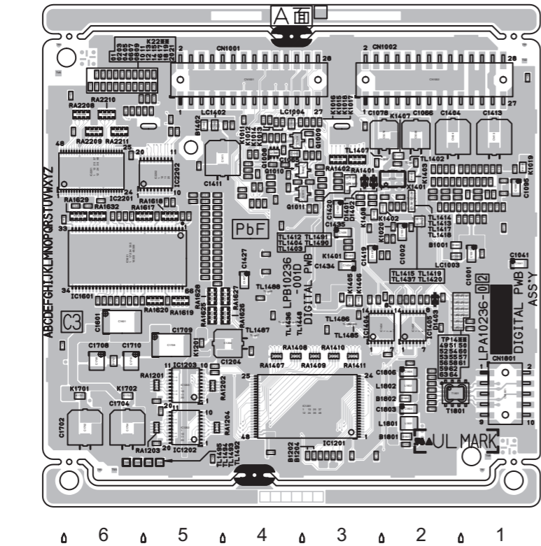
<02> DIGITAL LPB10236-001D -COMPONENT SIDE-
